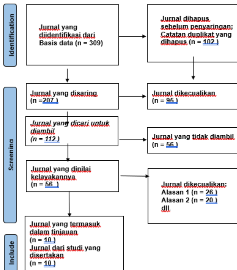
Gambar 01. Flowchart Prisma
